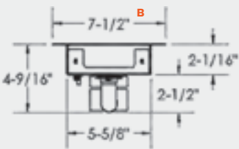
End View
